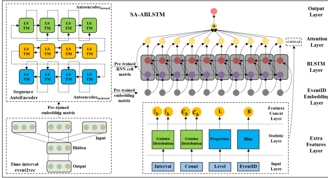
Figure 5: SA-ABLSTM architecture
